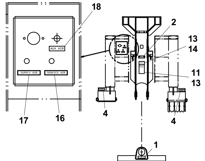
VIEW B-B
