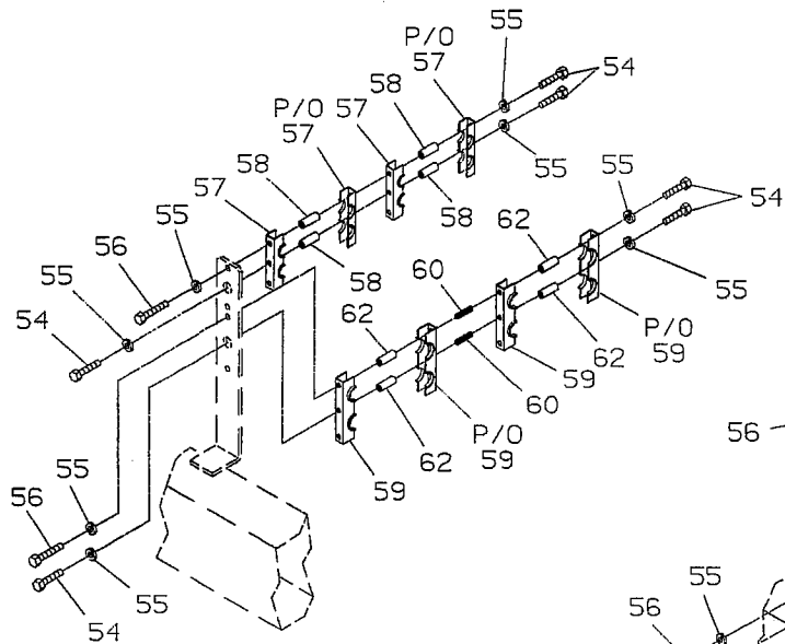
VIEW A
