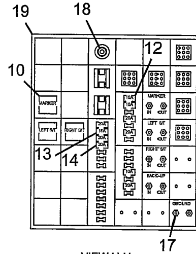
VIEW H-H
