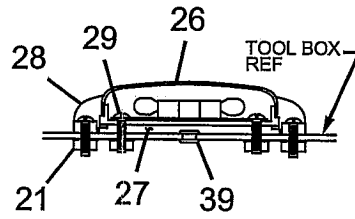
VIEW E-E
