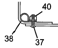
VIEW M-M
