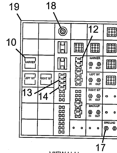
VIEW H-H
