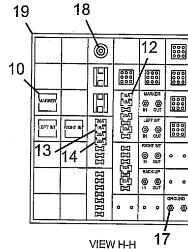
VIEW H-H
