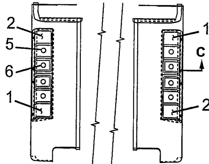
VIEW B-B
