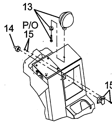
VIEW D
