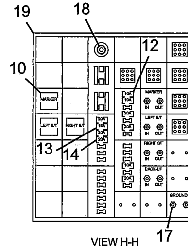
VIEW H-H
