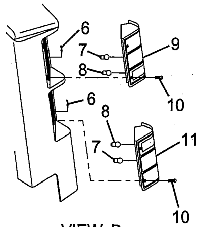
VIEW B
