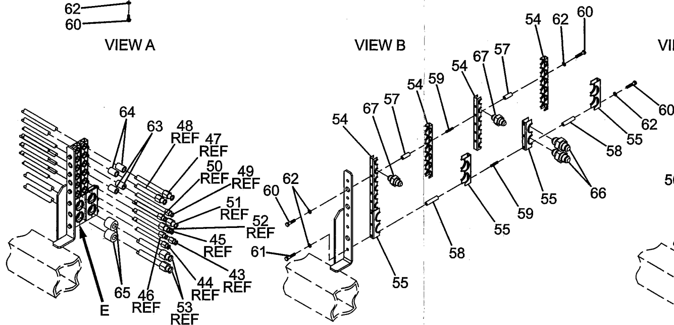
VIEW D
