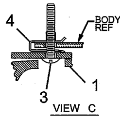
VIEW C
