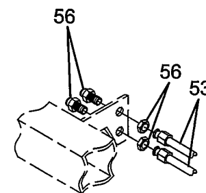
VIEW F
