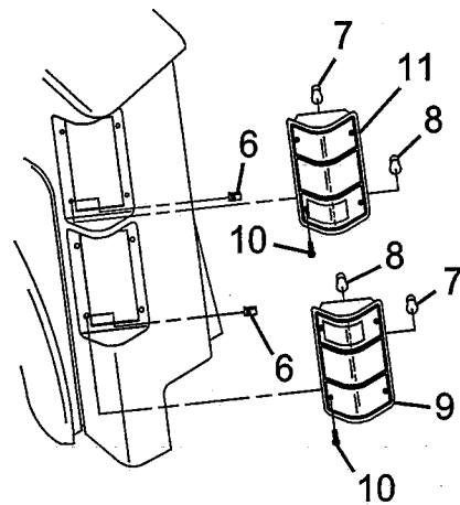
VIEW E
